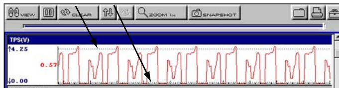
Figure 5-31 Sample set trigger levels
