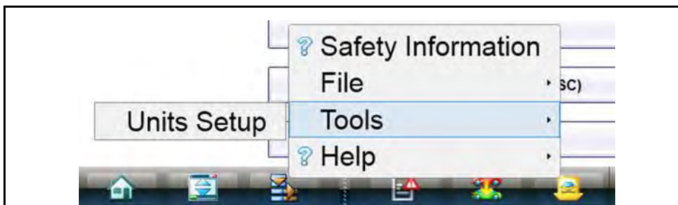
Figure 3-7 Menu icon
