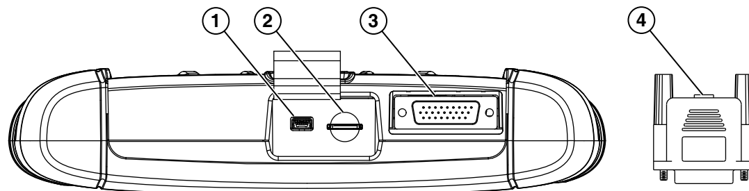
Figure 2-2 Top view
